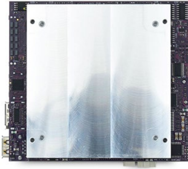
Bottom side showing heat spreader mounting plate
